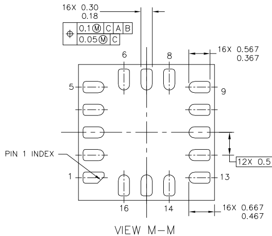
VIEW M-M
